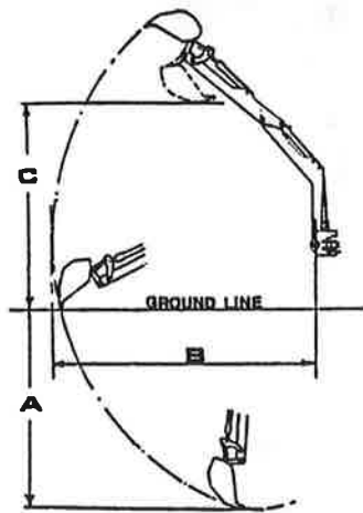
OPERATING DIAGRAM
