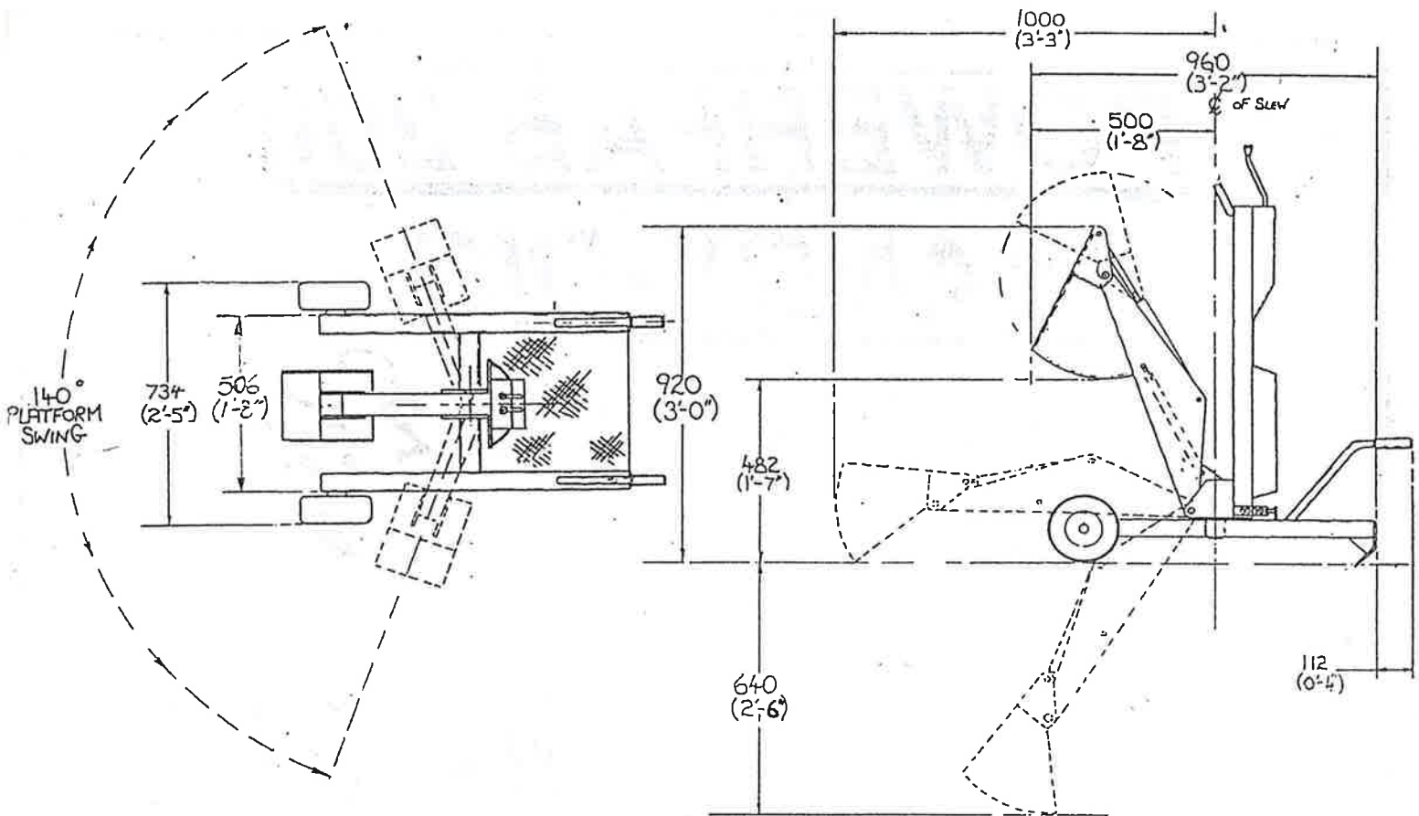
OPERATING DIAGRAM AND MAJOR DIMENSIONS
